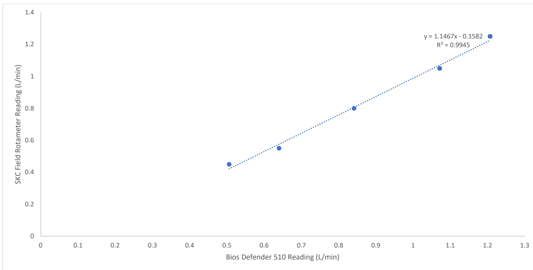
Figure 33. SKC Field Rotameter Calibration Curve
